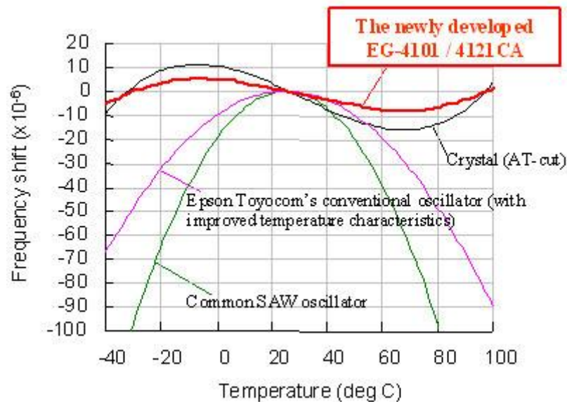
Figure 1. Frequency-Temperature Coefficient Comparison
